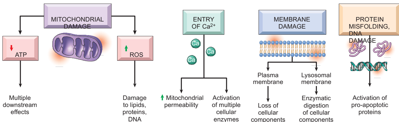
Figure 1-14 The principal biochemical mechanisms and sites of damage in cell injury. ATP, adenosine triphosphate; ROS, reactive oxygen species.
