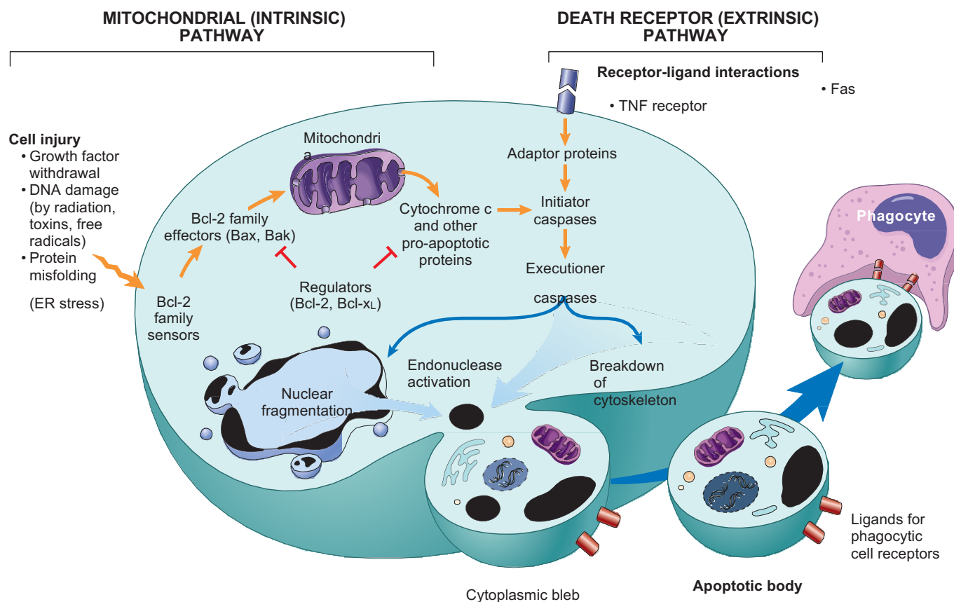
Figure 1–22 Mechanisms of apoptosis. The two pathways of apoptosis differ in their induction and regulation, and both culminate in the activation of caspases. In the mitochondrial pathway, proteins of the Bcl-2 family, which regulate mitochondrial permeability, become imbalanced and leakage of various substances from mitochondria leads to caspase activation. In the death receptor pathway, signals from plasma membrane receptors lead to the assembly of adaptor proteins into a “death-inducing signaling complex,” which activates caspases, and the end result is the same.
