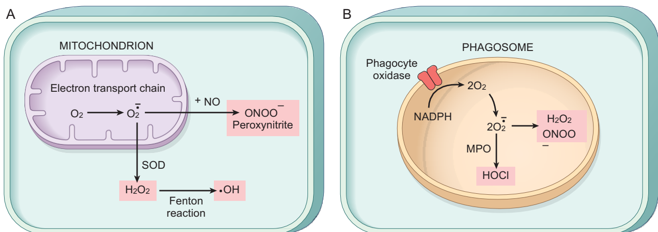
Figure 1-18 Pathways of production of reactive oxygen species. A , In all cells, superoxide ( O_2^- ) is generated during mitochondrial respiration by the electron transport chain and may be converted to H_2O_2 and the hydroxyl ( \cdot OH ) free radical or to peroxynitrite ( ONOO^- ). B , In leukocytes (mainly neutrophils and macrophages), the phagocyte oxidase enzyme in the phagosome membrane generates superoxide, which can be converted to other free radicals. Myeloperoxidase (MPO) in phagosomes also generates hypochlorite from reactive oxygen species (ROS). NO, nitric oxide; SOD, superoxide dismutase.
