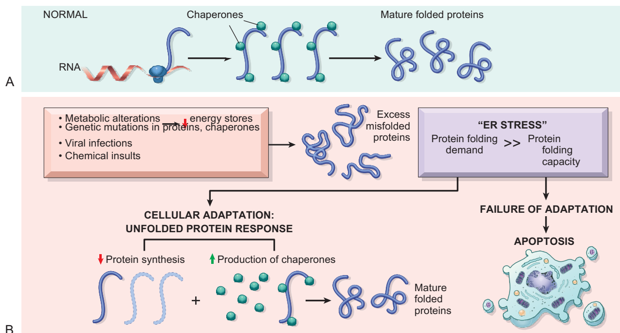
Figure 1–24 The unfolded protein response and ER stress. A , In healthy cells, newly synthesized proteins are folded with the help of chaperones and are then incorporated into the cell or secreted. B , Various external stresses or mutations induce a state called ER stress, in which the cell is unable to cope with the load of misfolded proteins. Accumulation of these proteins in the ER triggers the unfolded protein response, which tries to restore protein homeostasis; if this response is inadequate, the cell dies by apoptosis.
